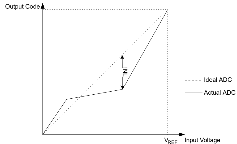
Figure 31-4. Integral Nonlinearity
