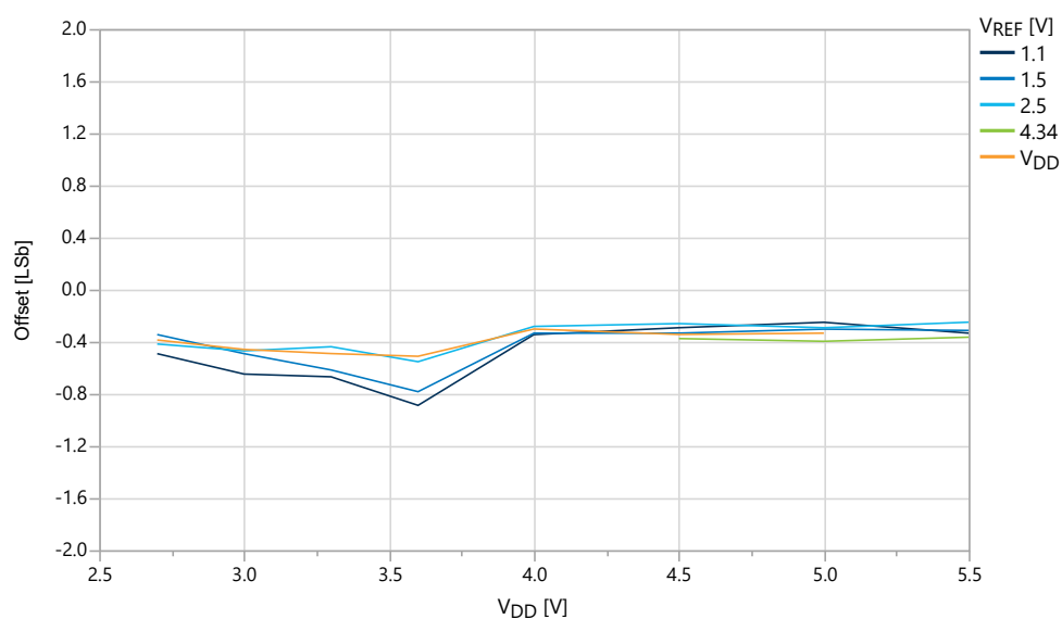
Figure 38-44. Offset Error vs. V_{DD} ( f_{ADC} = 115 kps) at T = 25^{\circ}C , REFSEL = Internal Reference
