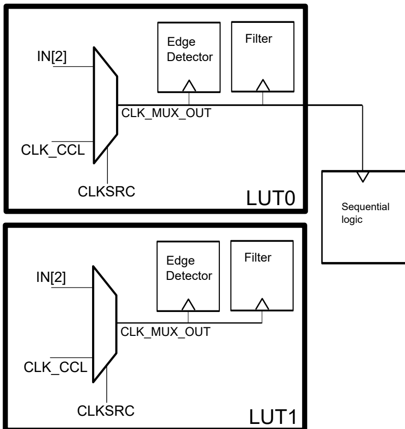
Figure 29-11. Clock Source Settings
