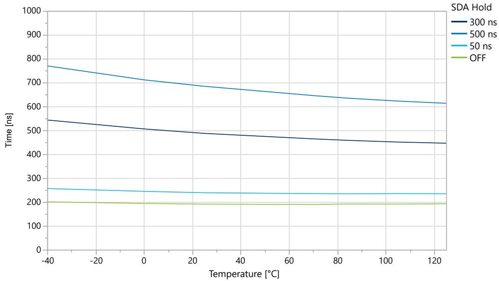
Figure 38-70. TWI SDA Hold Time vs. Temperature (Slave Mode) V_{DD} = 3V , CLK_{CPU} = 10\text{ MHz}
