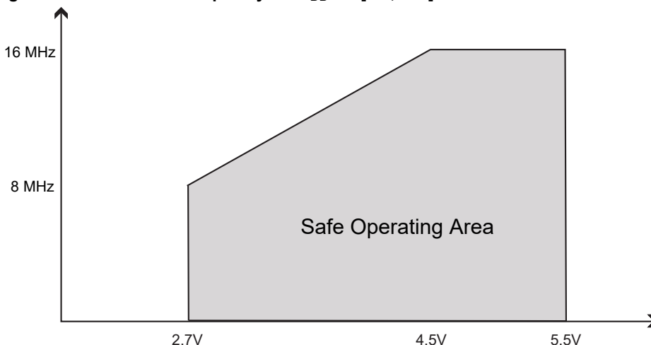
Figure 37-1. Maximum Frequency vs. V_{DD} for [-40, 125]^{\circ}C
