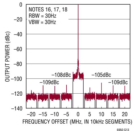
PECLx Spurious Response f_{VCO} = 125MHz , f_{PDF} = 5MHz
