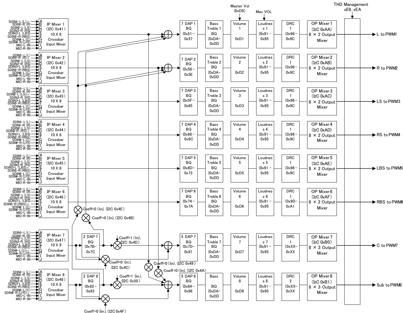
Figure 23. TAS5548 DAP Architecture With I²C Registers ( f_s \leq 96 kHz)
