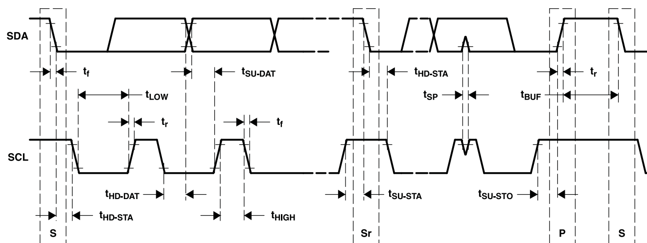
Figure 1. SCL and SDA Timing
