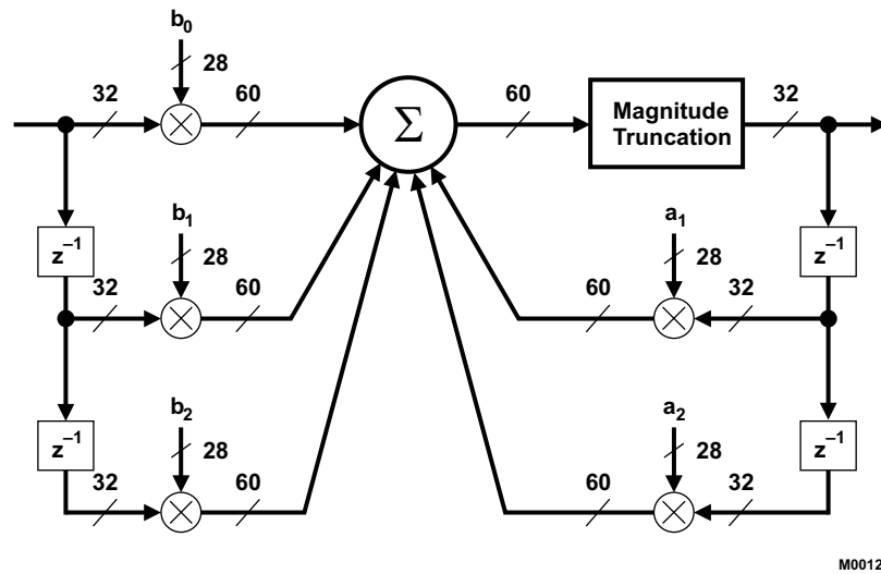
Figure 33. Biquad Filter Structure
