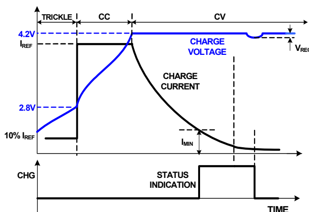
FIGURE 1. TYPICAL CHARGE CYCLE WITH TIMEOUT
