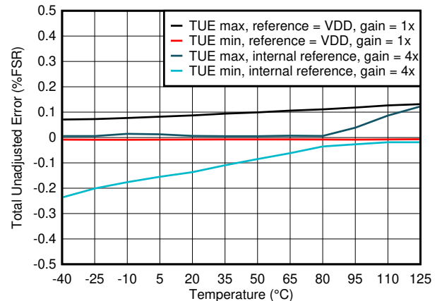
Figure 7-16. Total Unadjusted Error vs Temperature
