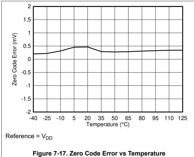
Figure 7-17. Zero Code Error vs Temperature
