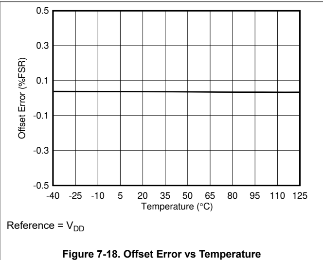
Figure 7-18. Offset Error vs Temperature
