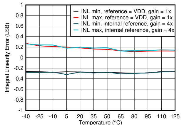
Figure 7-14. Integral Linearity Error vs Temperature
