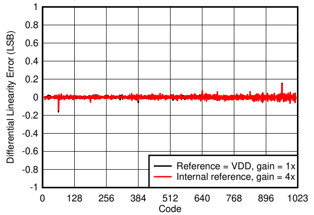
Figure 7-12. Differential Linearity Error vs Digital Input Code
