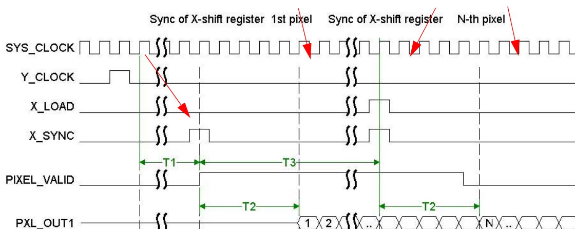
Figure 23. Pixel Output
