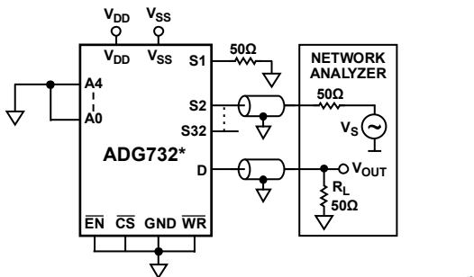
Figure 23. Channel-to-Channel Crosstalk
