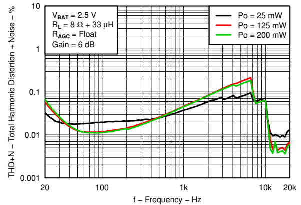
Figure 7-8. Total Harmonic Distortion + Noise vs Frequency
