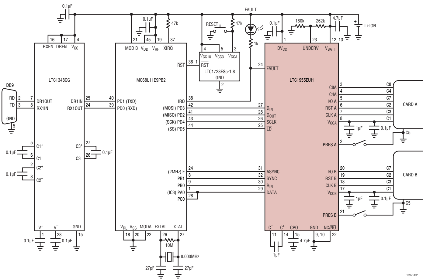
Battery-Powered RS232 to Dual Smart Card Interface
