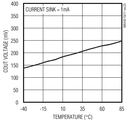
COMPARATOR OUTPUT VOLTAGE ( V_{OL} ) vs. TEMPERATURE
