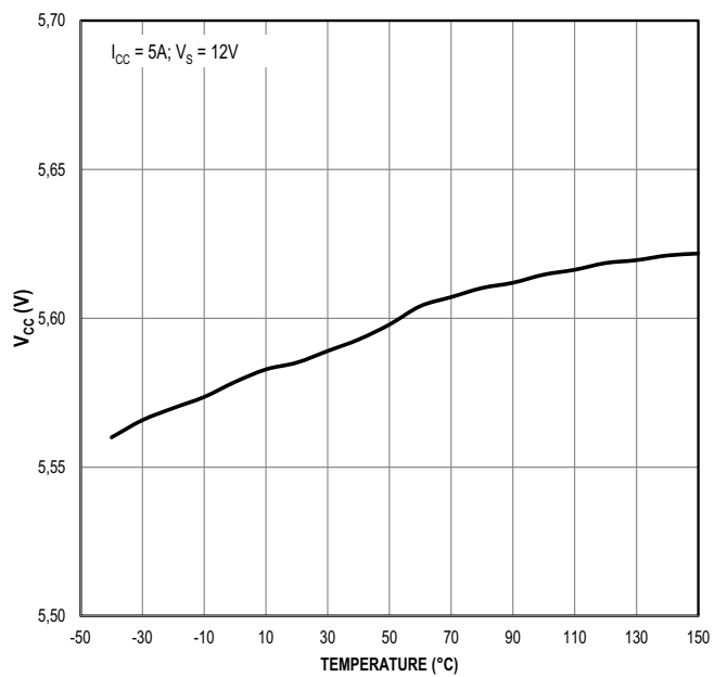
V_{\text{CC}} versus Temperature
