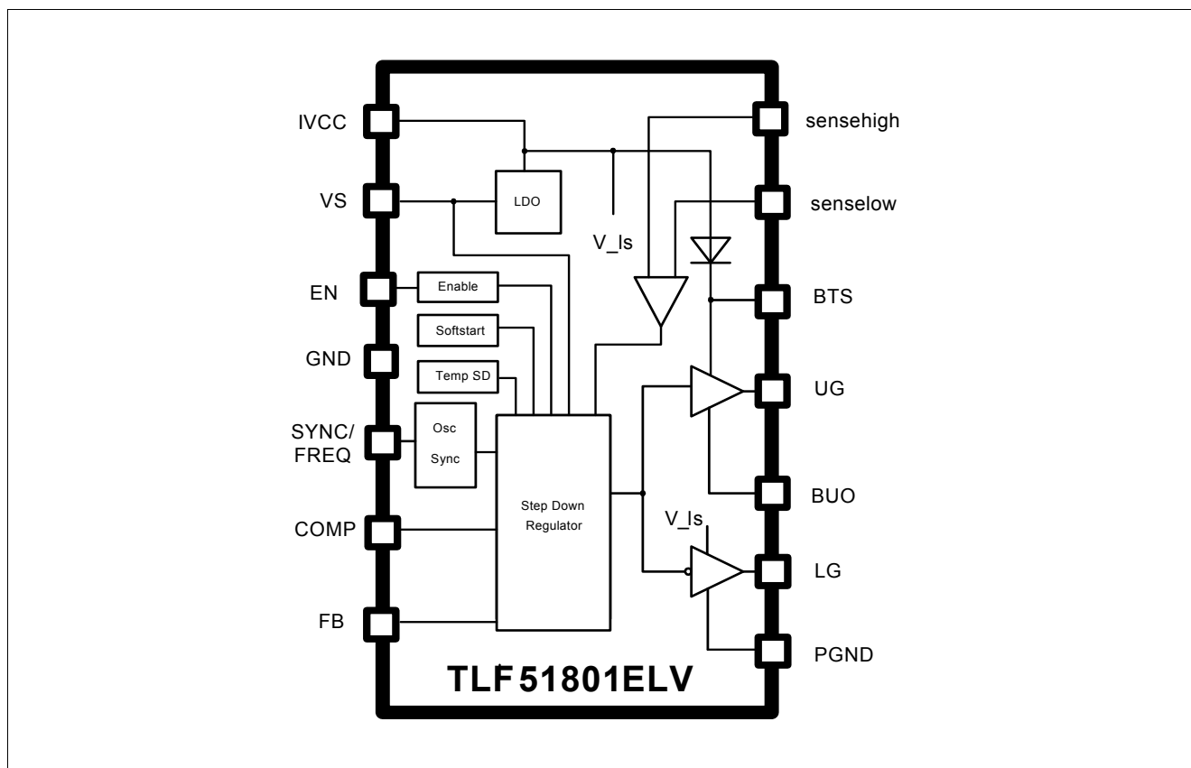
Figure 1 Block Diagram
