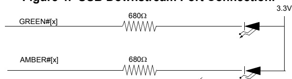
Figure 4. USB Downstream Port Connection.
