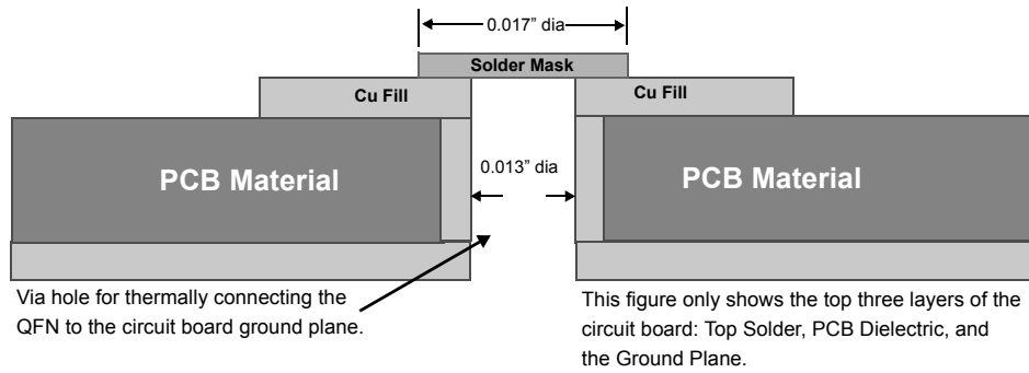
Figure 9. Cross section of the Area Underneath the QFN Package
