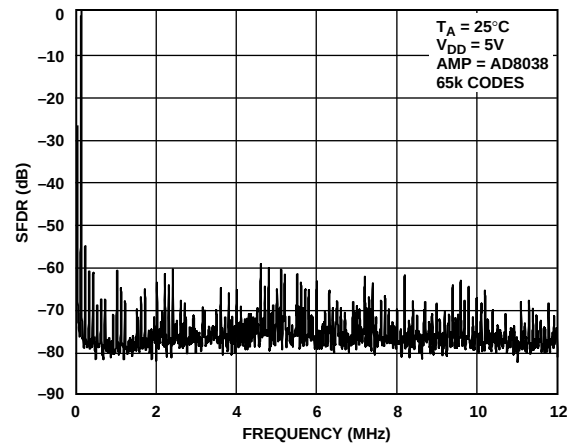
图29. 宽带SFDR, f_{OUT} = 100 kHz, 时钟 = 25 MHz
