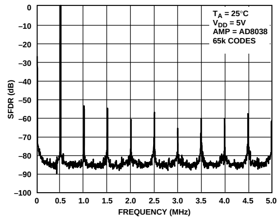
图30. 宽带SFDR, f_{OUT} = 500 kHz, 时钟 = 10 MHz
