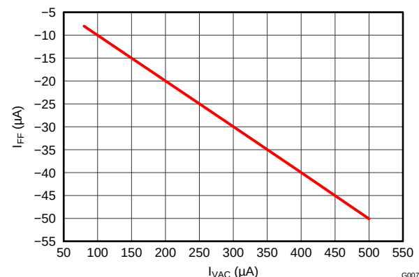
Figure 6. Feedforward Source Current ( I_{\text{FF}} ) vs. VAC Current ( I_{\text{VAC}} )
