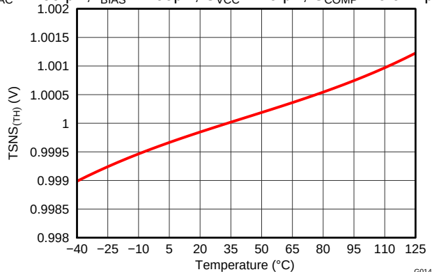
Figure 13. Thermal Foldback Threshold vs. Junction Temperature
