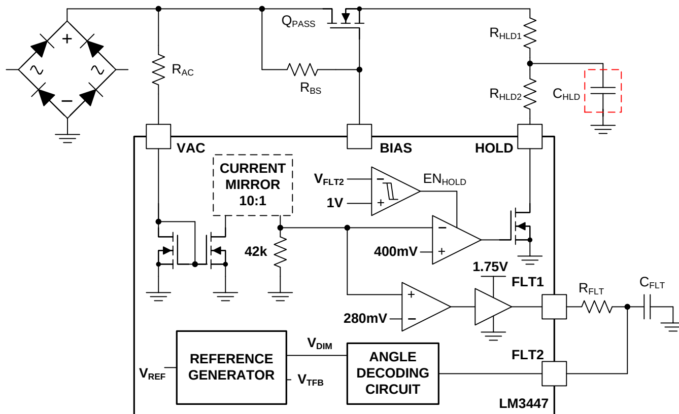
Figure 27. Phase Angle Detection and HOLD Current Circuit
