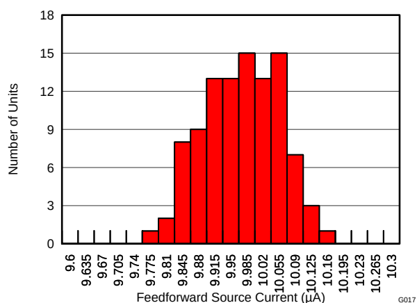
Figure 16. Feedforward Source Current (I FF ) Variation (I VAC =100μA, Temperature = 25°C)
