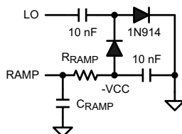
Figure 39. R_{RAMP} to -VCC for V_{OUT} < 7.5\text{ V}
