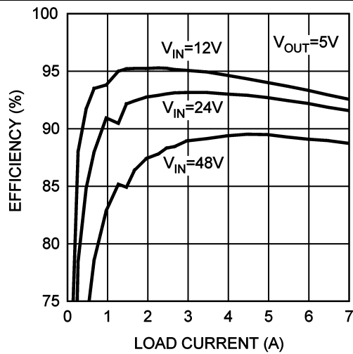
Figure 40. Efficiency With 6-μH Copper Inductor
