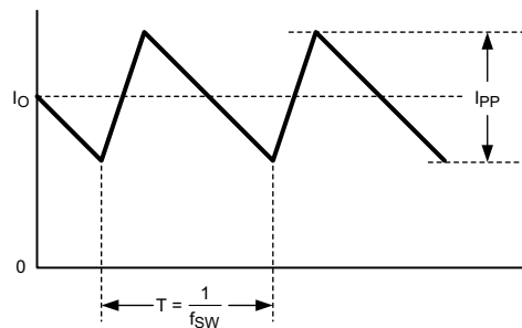
Figure 34. Inductor Current
