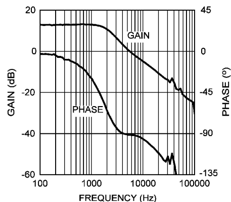
Figure 35. Modulator Gain and Phase
