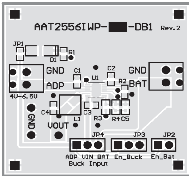
Figure 6: AAT2556 Evaluation Board Top Side Layout.
