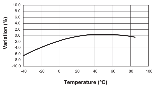
Switching Frequency Variation
