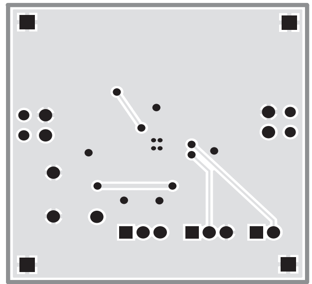
Figure 7: AAT2556 Evaluation Board Bottom Side Layout.
