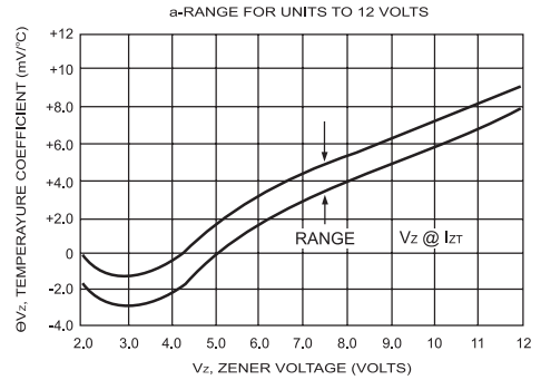
FIG.7- TEMPERATURE COEFFICIENTS
