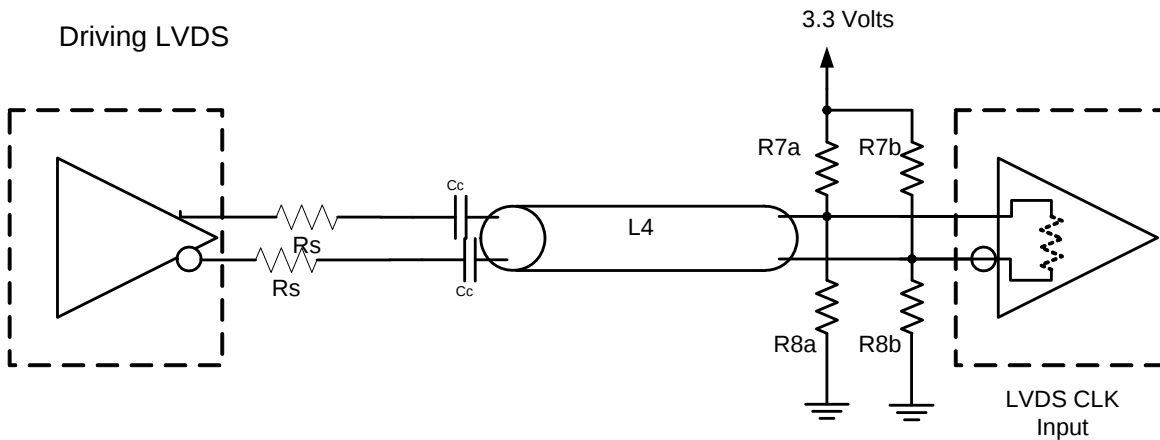
Driving LVDS inputs
