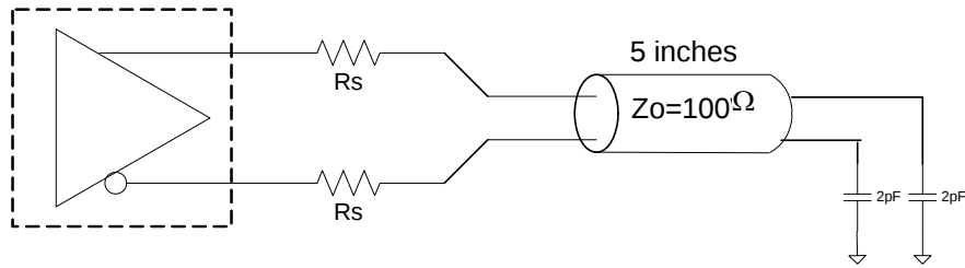
Low-Power Differential Output Test Load
