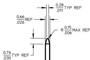
DETAIL Y SCALE 5:1 SEE NOTE 10
