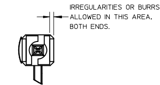
DETAIL Z SCALE 5:1
