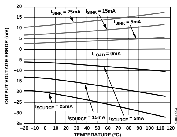
Figure 3. Output Voltage Error vs. Temperature
