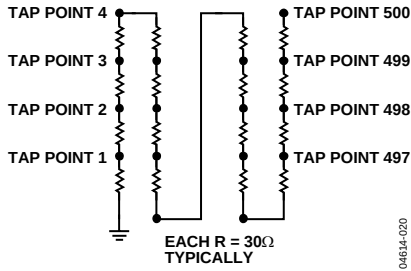
Figure 20. 500 Mask-Programmable Resistor String
