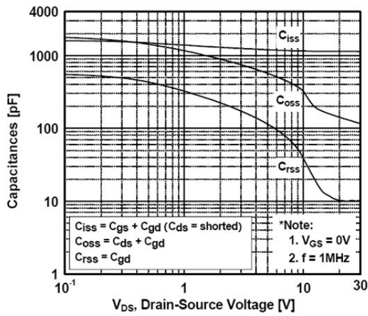
Fig. 5 Capacitance Characteristics
