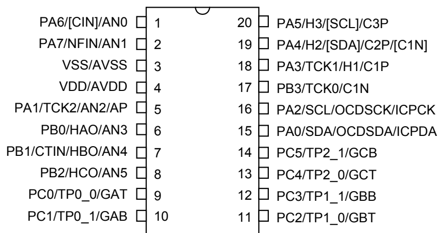
HT66FM5230 20SSOP-A
