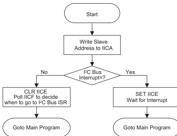
I²C Bus Initialisation Flow Chart
