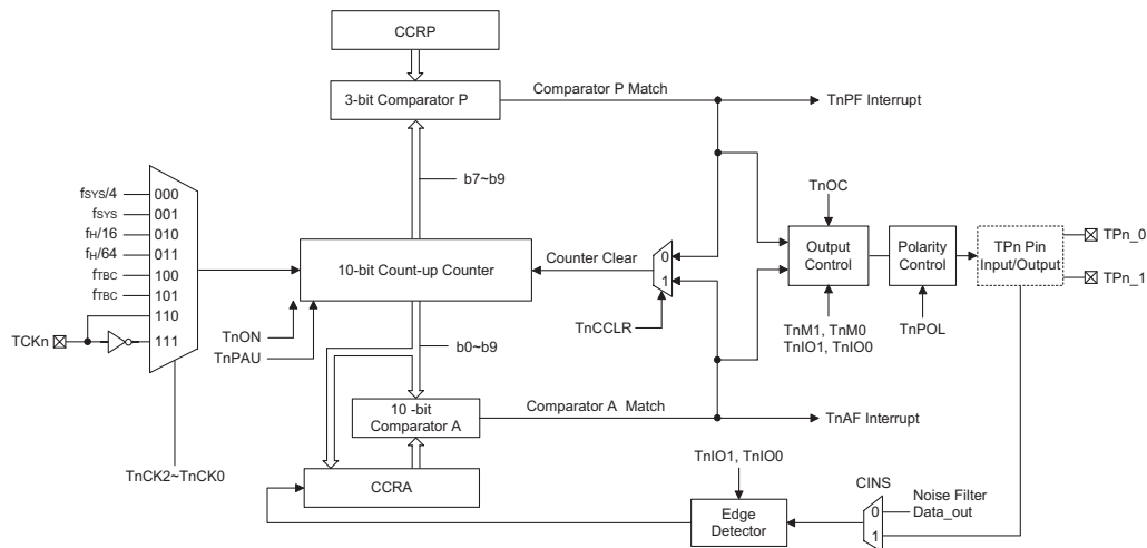
Standard Type TM Block Diagram (n=2)
