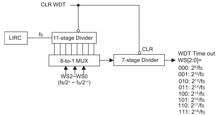
Watchdog Timer
