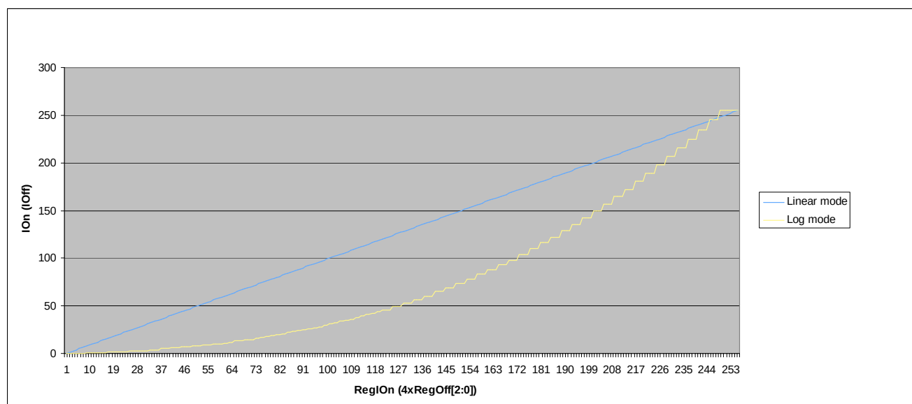
Figure 17 – LED Driver Linear vs Logarithmic Function (II)
