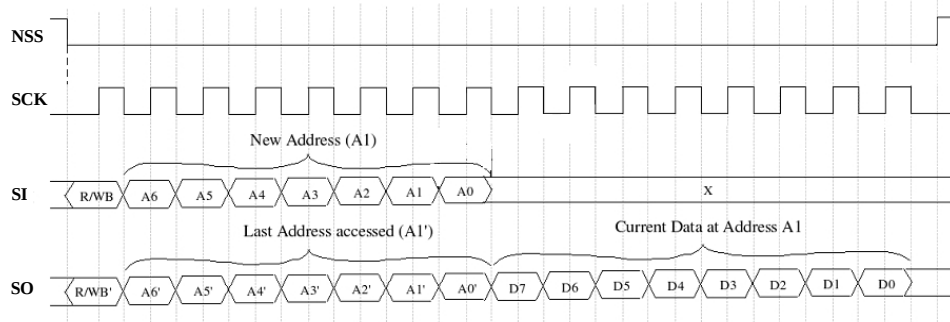
Figure 8 – SPI Read Operation
