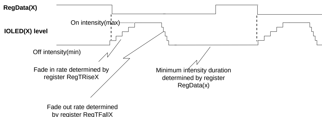
Figure 15 – LED Driver Single Shot Mode
