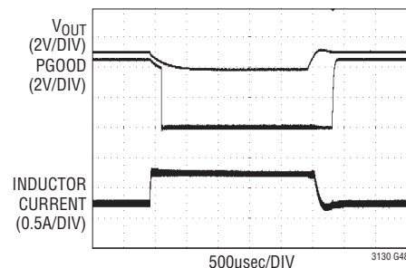
PGOOD Response to a Drop in V_{OUT} Due to a Step Overload
