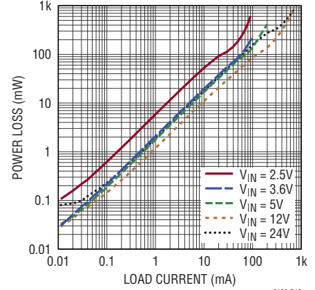
Power Loss, V_{OUT} = 12V , Burst Mode Operation (LTC3130-1)
