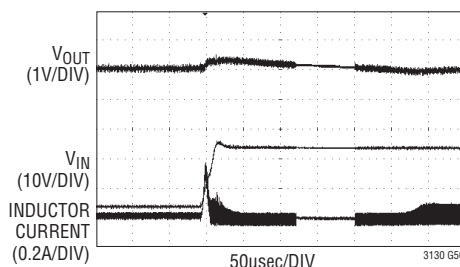
V_{IN} Line Step Response in Fixed Frequency
