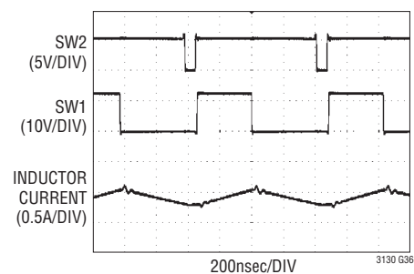
Fixed Frequency PWM Waveforms (Buck Region)
