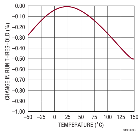
Accurate RUN Threshold vs Temperature (Normalized to 25^\circ\text{C} )
