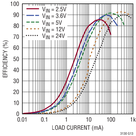
Efficiency, V_{OUT} = 15V (LTC3130)
