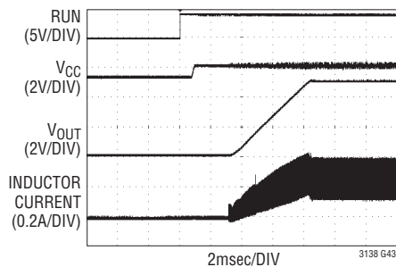
Start-Up Sequence When Raising RUN Pin ( V_{IN} = 12\text{V} )
