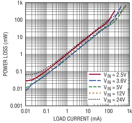
Power Loss, V_{OUT} = 5V , Burst Mode Operation (LTC3130-1)
