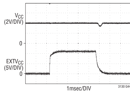
V_{CC} Response to a Step on EXT V_{CC} ( V_{IN} > 4\text{V} )
