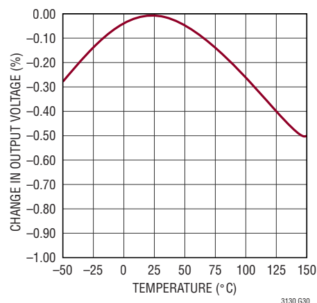
Output Voltage vs Temperature LTC3130-1 (Normalized to 25^\circ\text{C} )
