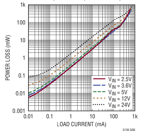
Power Loss, V_{OUT} = 1.8\text{V} , Burst Mode Operation (LTC3130-1)
