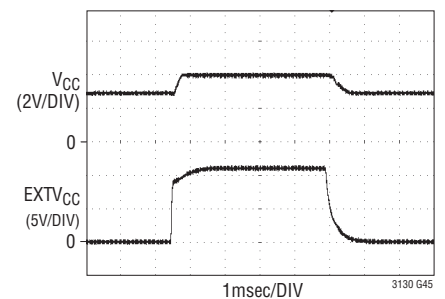
V_{CC} Response to a Step on EXT V_{CC} ( V_{IN} = 3\text{V} )
