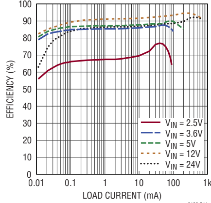
Efficiency, V_{OUT} = 12V , Burst Mode Operation (LTC3130-1)
