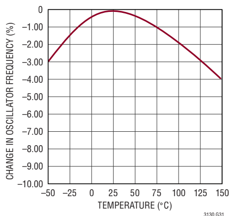
Oscillator Frequency vs Temperature (Normalized to 25^\circ\text{C} )
