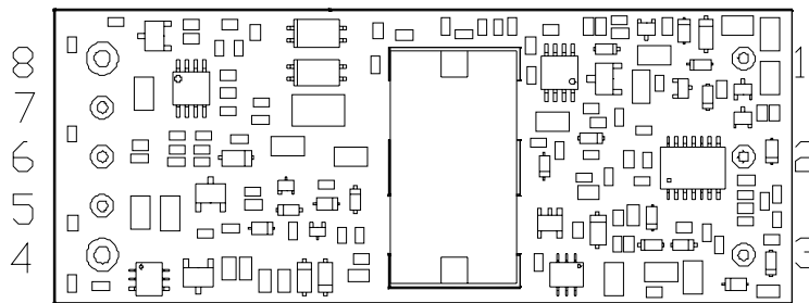
BOTTOM VIEW
