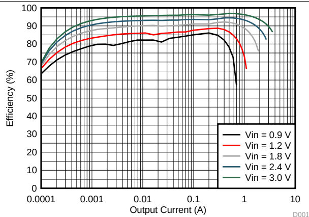
图 1. Load Efficiency with Different Input
