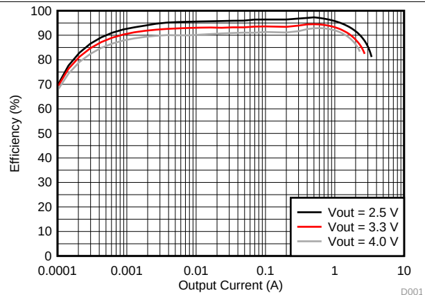
图 2. Load Efficiency with Different Output
