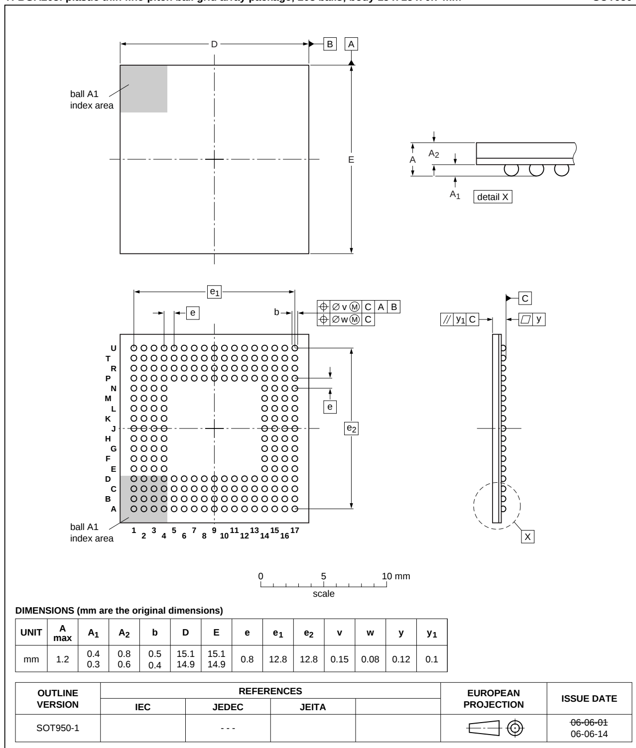
Fig 42. TFBGA208 package
