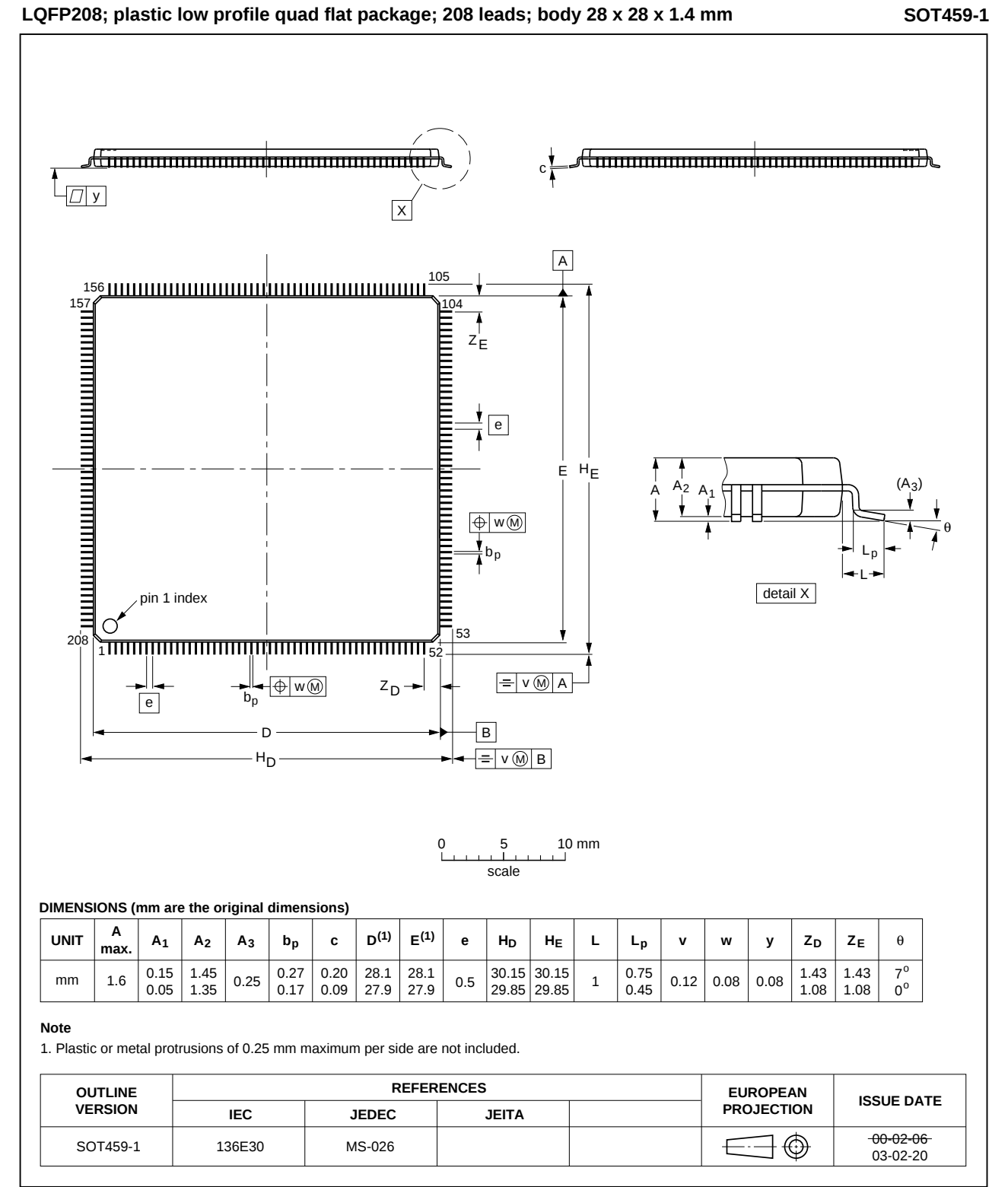
Fig 41. LQFP208 package
