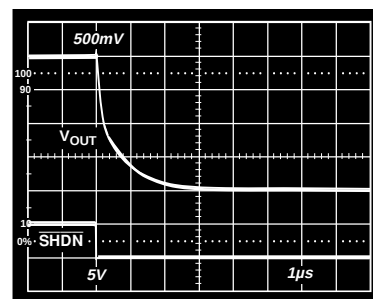
Figure 21. Shutdown Time
