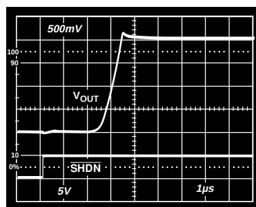
Figure 20. Shutdown Recovery Time
