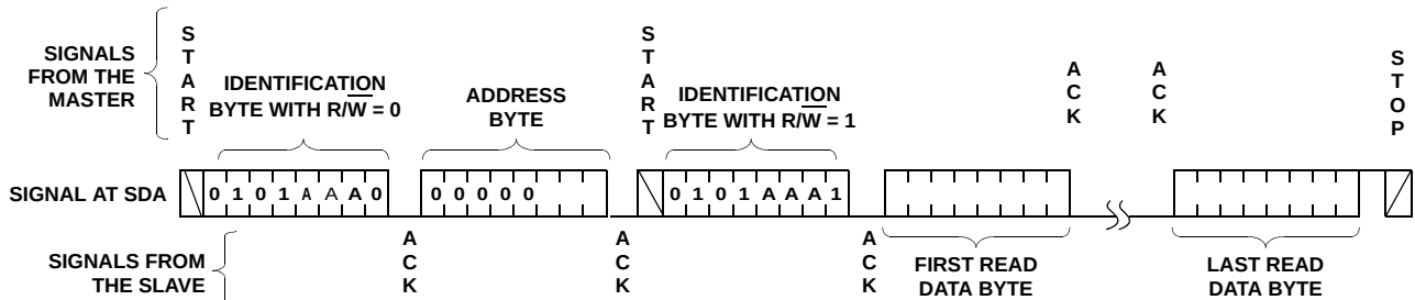
FIGURE 18. RANDOM ADDRESS READ SEQUENCE
