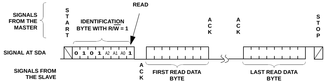
FIGURE 17. ADDRESS READ SEQUENCE
