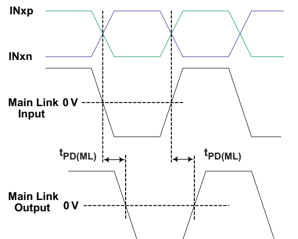
Figure 5. Main Link Delay Measurements
