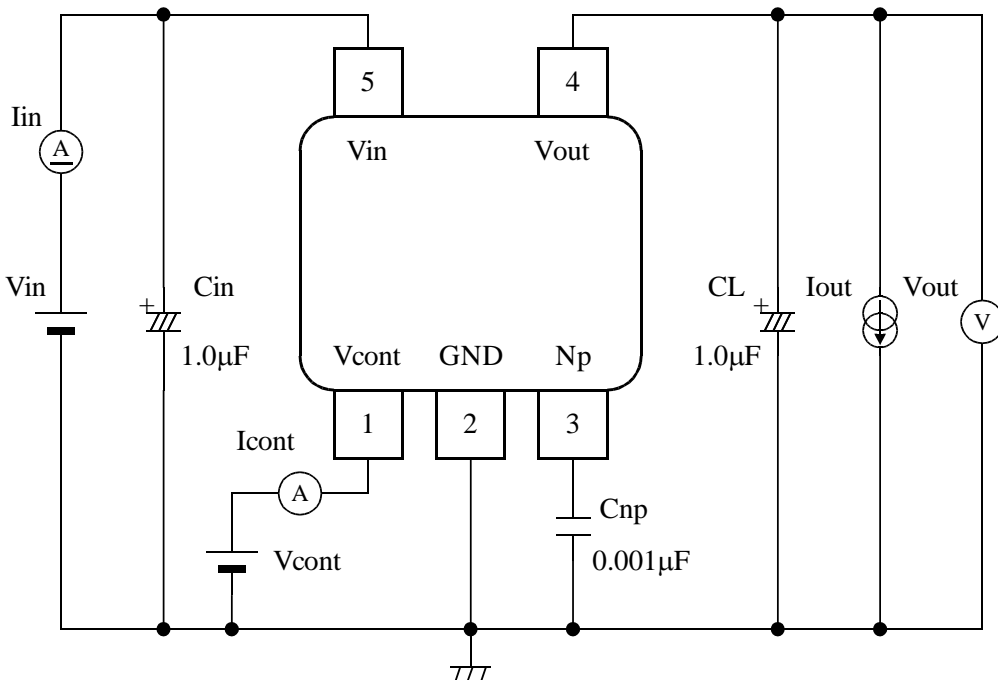
Figure 9. Test Circuit
