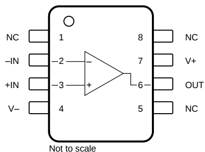
Pin Functions: TLV172
