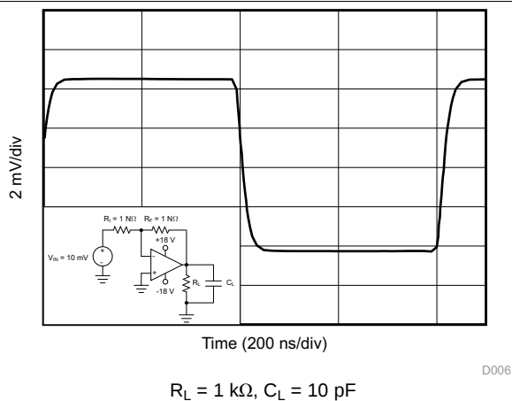
Figure 17. Small-Signal Step Response (10 mV)
