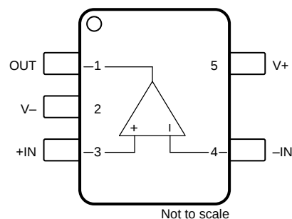
TLV172: DBV Package 5-Pin SOT-23 Top View
