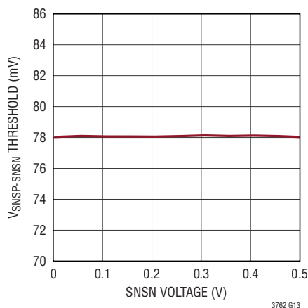
V_{\text{SNSP-SNSN}} Current Limit Threshold vs SNSN Voltage, \text{SNSN} < 0.5\text{V}
