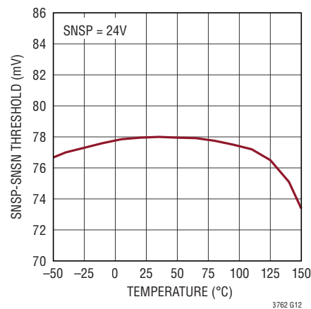
SNSP-SNSN Current Limit Threshold vs Temperature
