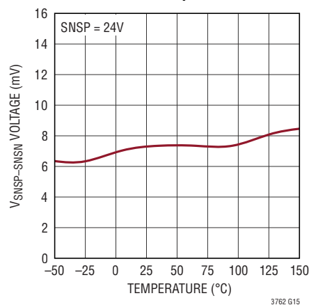
SNSP-SNSN Zero Cross Threshold vs Temperature
