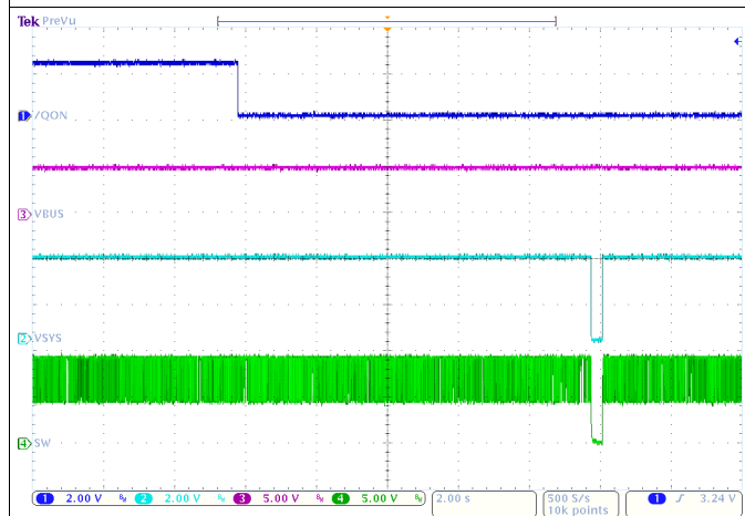
Figure 40. Power Up
