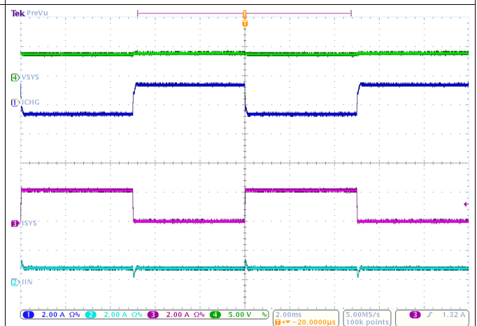
Figure 41. System Reset by \overline{QON} without VBUS Present
