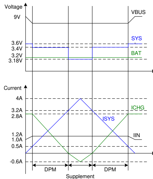
Figure 12. DPM Response
