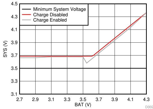
Figure 11. System Voltage vs Battery Voltage
