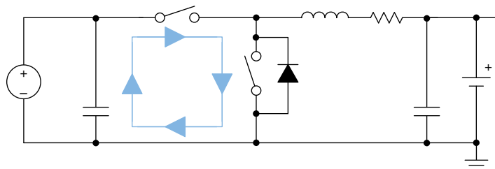
Figure 47. High Frequency Current Path
