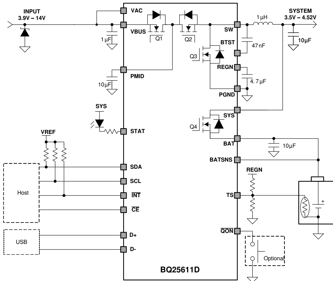
Figure 39. BQ25611D Application Diagram
