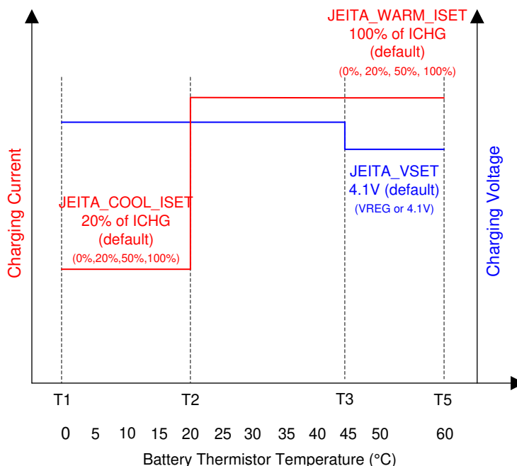
Figure 14. JEITA Profile
