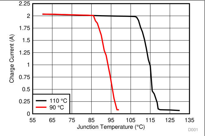
Figure 10. Charge Current vs Junction Temperature
