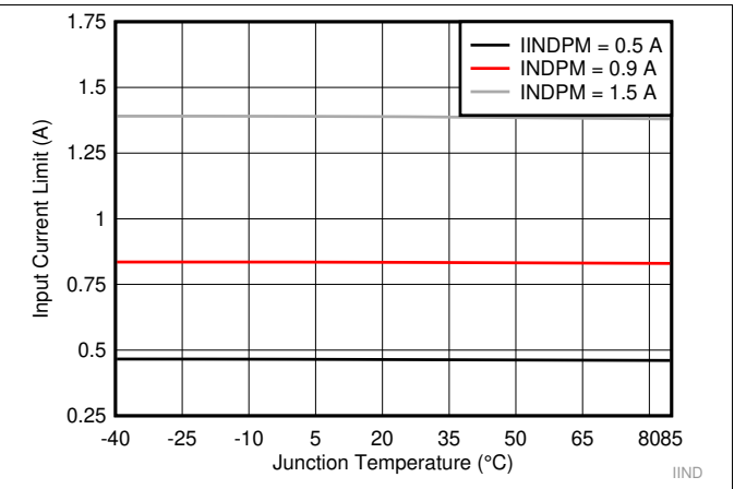
Figure 8. Input Current Limit vs Junction Temperature
