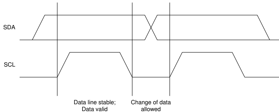
Figure 17. Bit Transfer on the I 2 C Bus
