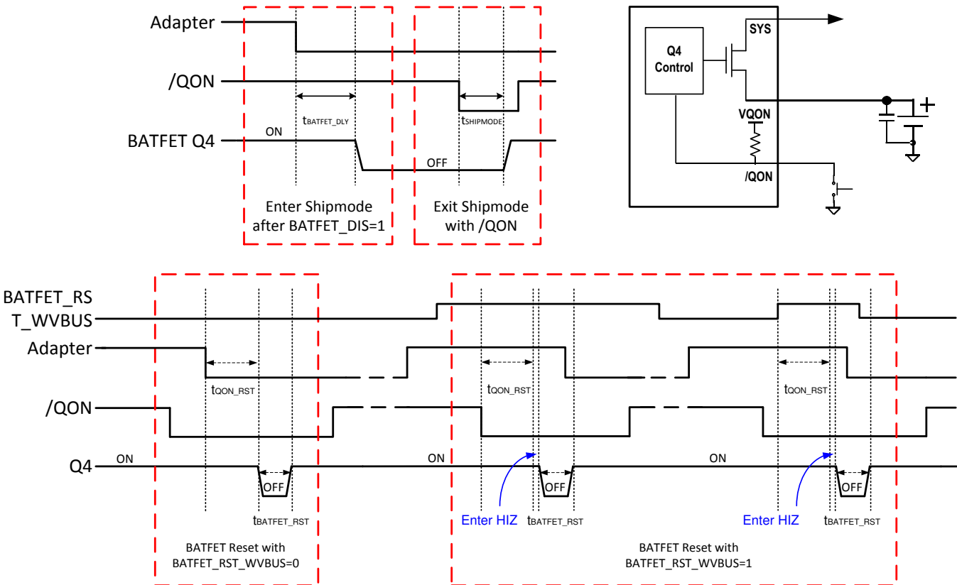
Figure 16. \overline{QON} Timing
