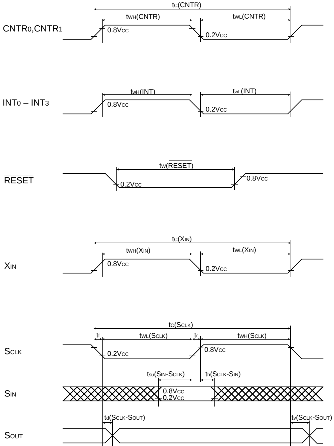
Fig. 46 Timing diagram
