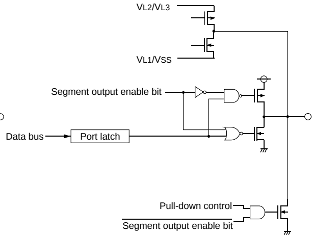
(2) Port P3
