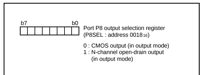
Fig. 9 Structure of port P8 output selection register
