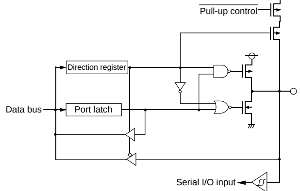
(6) Port P44
