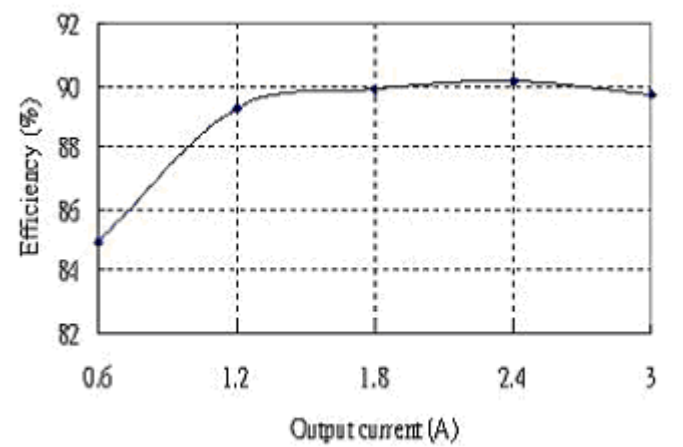
Figure 4: Converter efficiency vs. output current (5Vin/1.5Vout)
