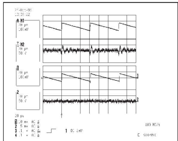
Figure 12 : Step Up Noise Reduction
