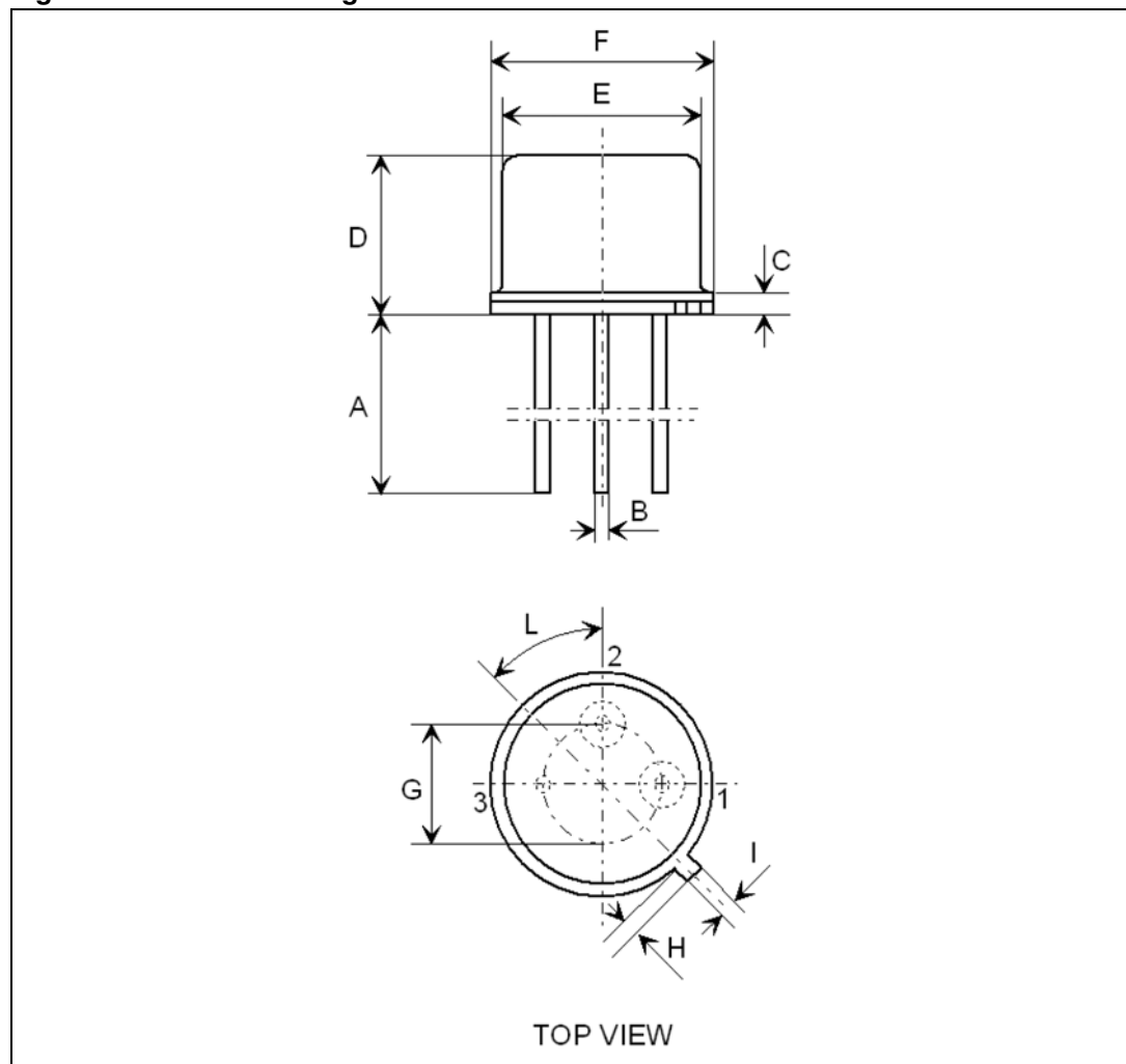
Figure 7. TO-39 drawing
