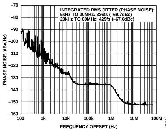
Figure 11. Absolute Phase Noise (Output Driver = LVPECL), f_{REF} = 8 kHz, f_0 = 155.52 MHz, LBW = 100 Hz, f_{SYSCLK} = 50 MHz (Crystal), PLL On
