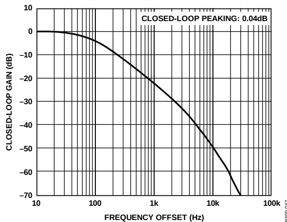
Figure 12. Jitter Transfer Bandwidth, Output Driver = LVPECL, f_{REF} = 19.44 MHz, f_0 = 155.52 MHz, LBW = 100 Hz (Phase Margin = 88°), f_{SYSCLK} = 1 GHz, PLL Off
