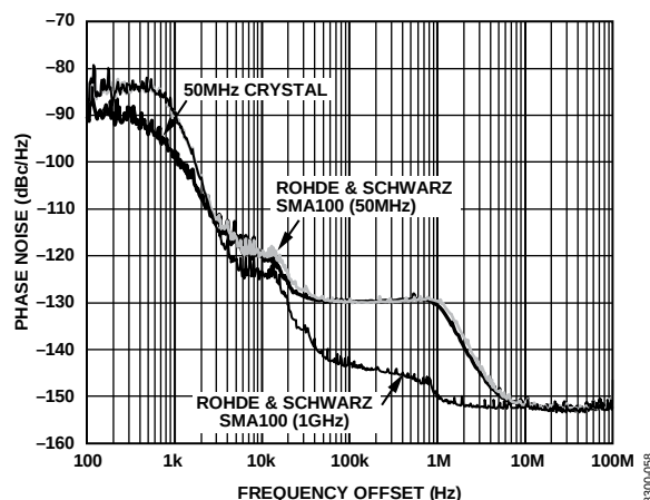
Figure 10. Absolute Phase Noise Comparison of SYSCLK Input Options (Output Driver = LVPECL), f_{REF} = 19.44 MHz, f_0 = 311.04 MHz, LBW = 1 kHz
