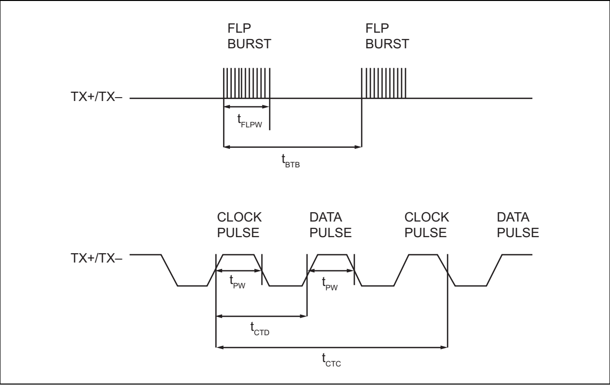
FIGURE 7-11: AUTO-NEGOTIATION TIMING DIAGRAM
