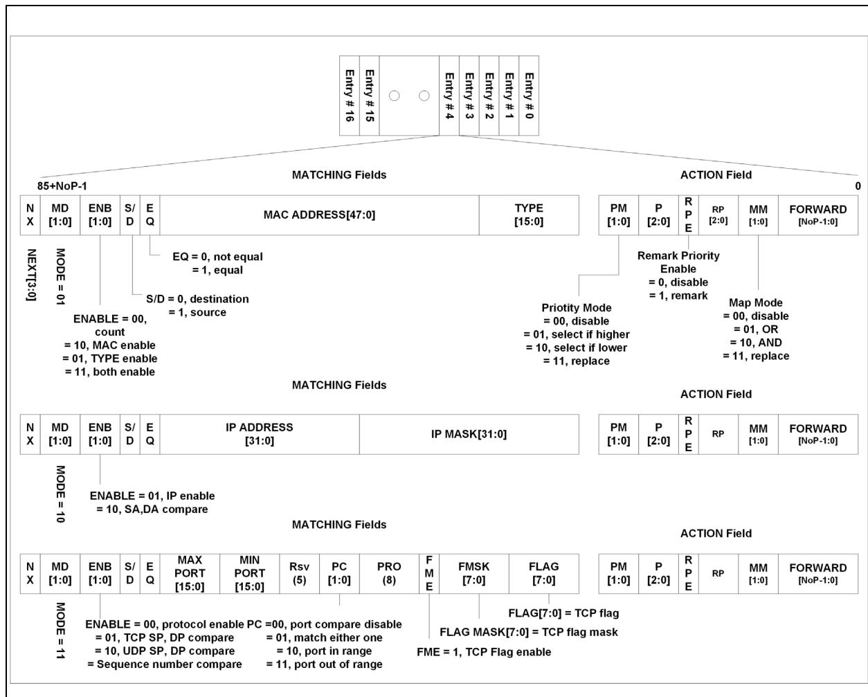
FIGURE 3-11: ACL FORMAT
