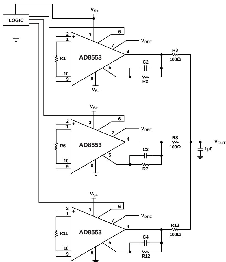
Figure 37. Multiplexed Output
