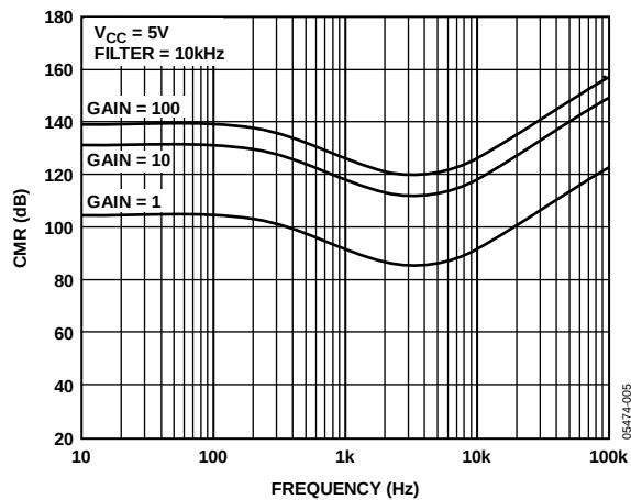
Figure 6. Common-Mode Rejection (CMR) vs. Frequency
