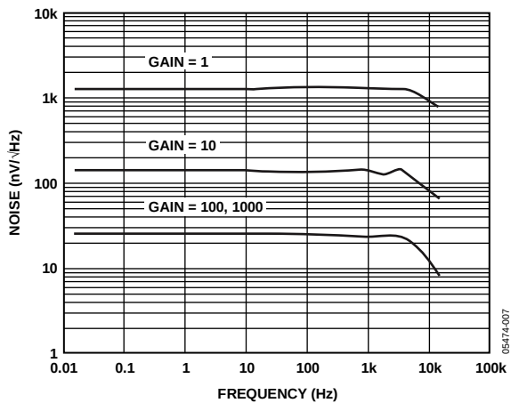
Figure 7. Voltage Noise Density
