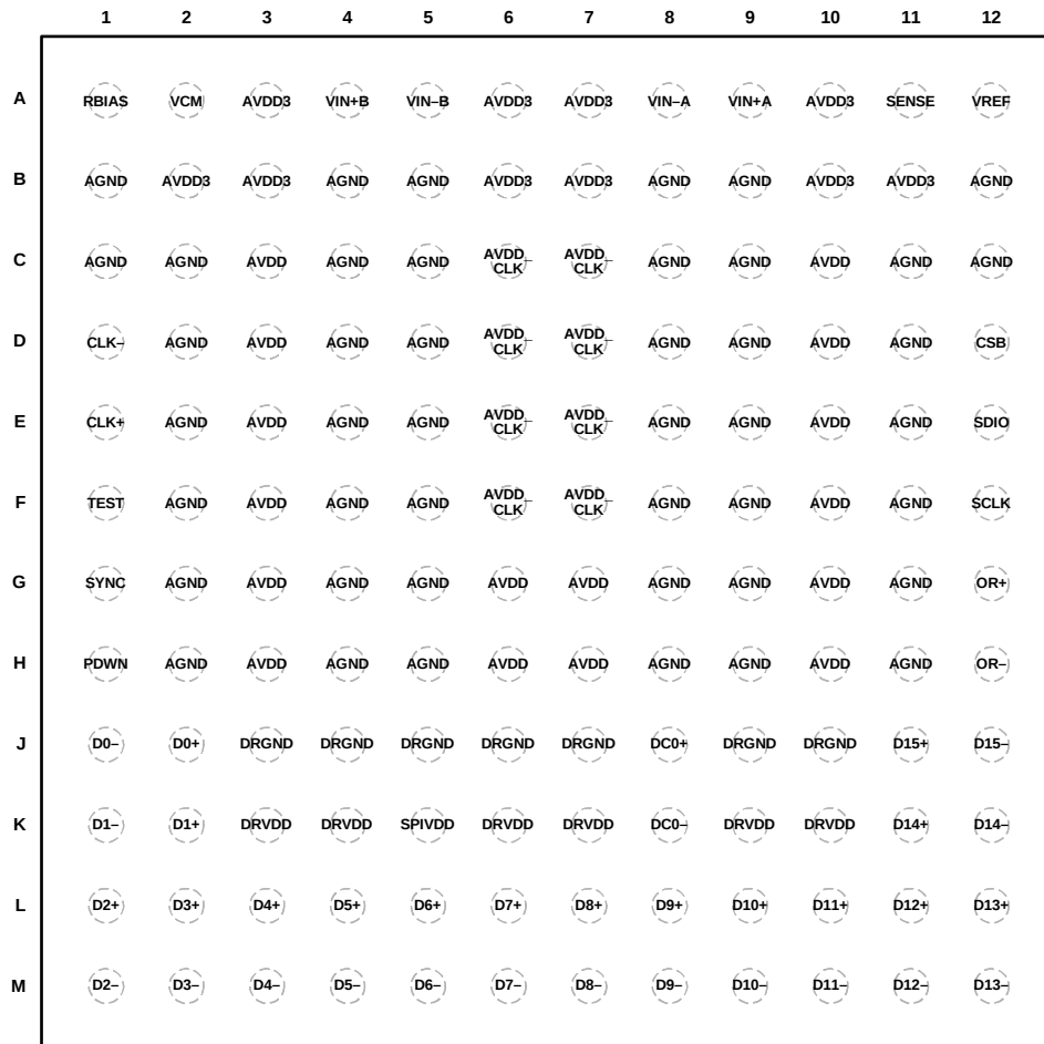
Figure 5. Pin Configuration
