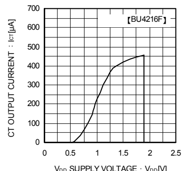
Fig.8 Ct Terminal Current
