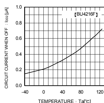
Fig.11 Circuit Current when OFF
