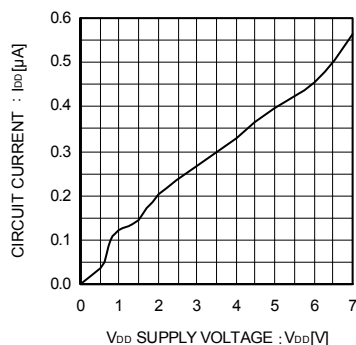
Fig.3 Circuit Current
