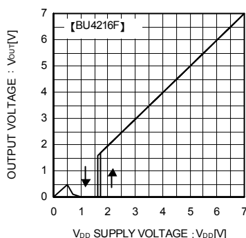
Fig.6 I/O Characteristics
