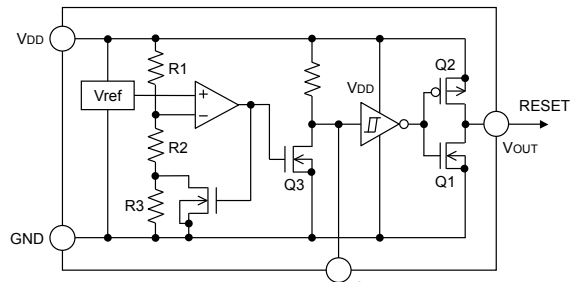
Fig.16 (BU43□□ type) internal block diagram
