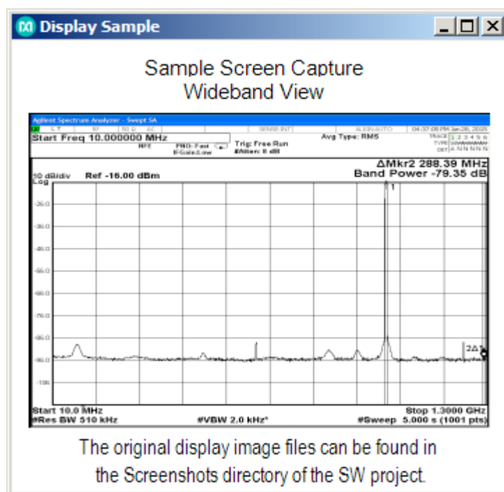
Figure 21. Test Tab Option for Displaying the Sample Wideband Spectrum Analyzer Capture
