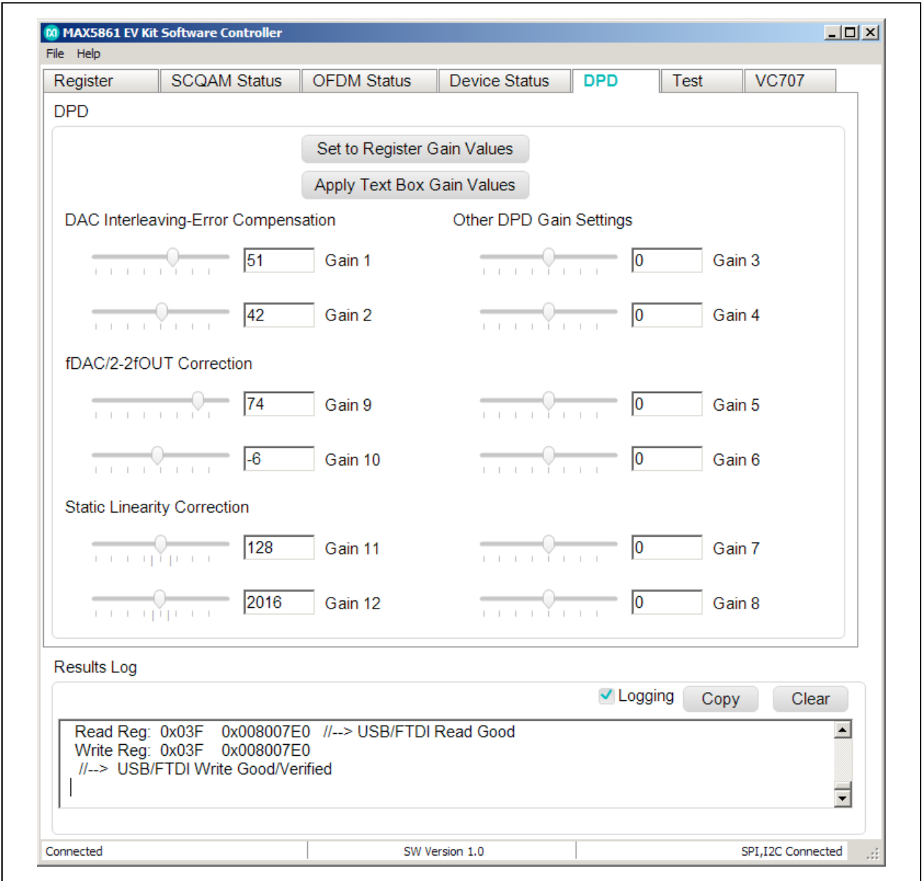
Figure 19. DPD Tab
