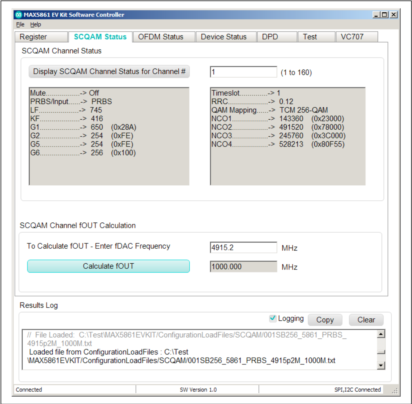
Figure 16. QAM Status Tab
