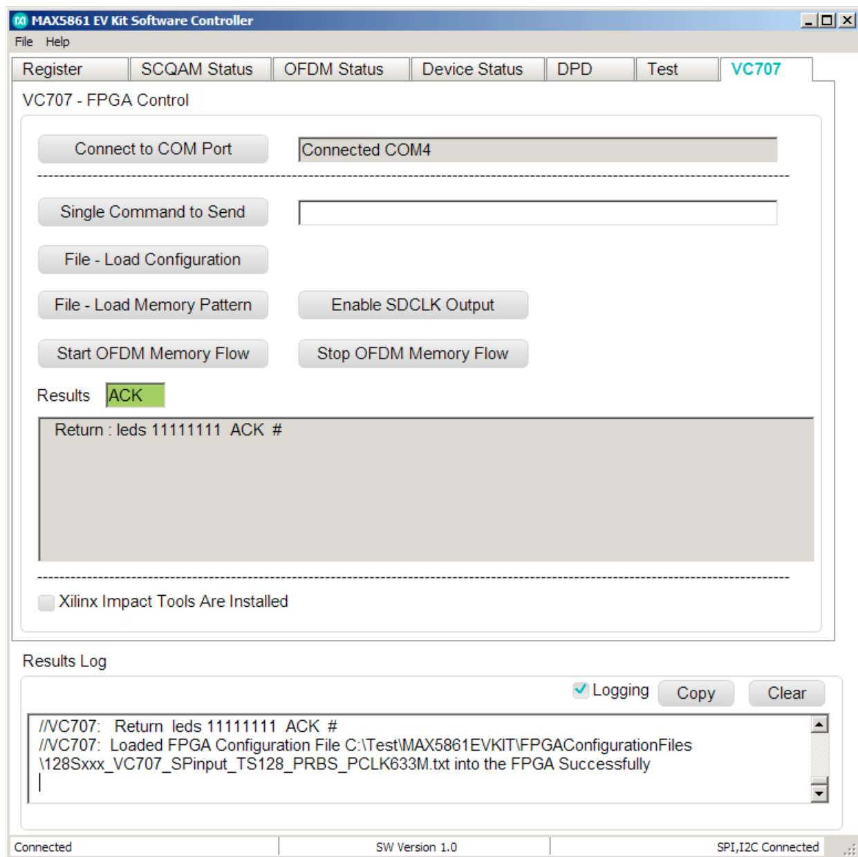
Figure 22. VC707 Tab
