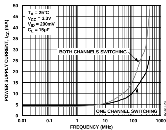
Figure 9. Power Supply Current vs. Frequency
