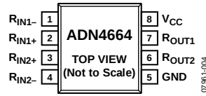
Figure 4. Pin Configuration
