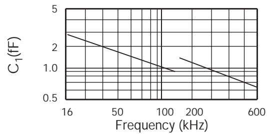
FIGURE 3 CX-2V TYPICAL QUALITY FACTOR (Q)
