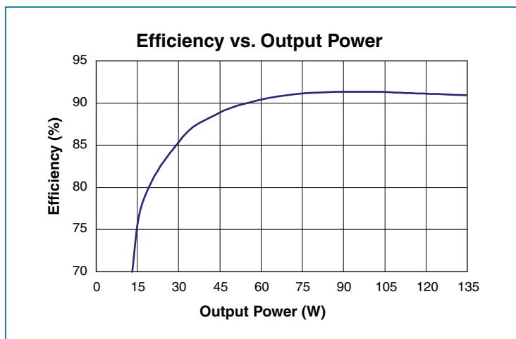
Figure 5 — Efficiency vs. output power
