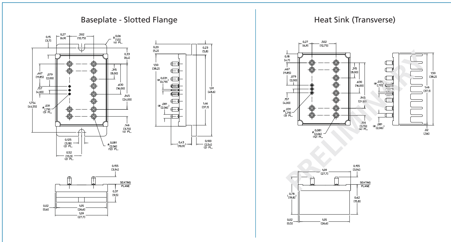
Figure 18 — Module outline
