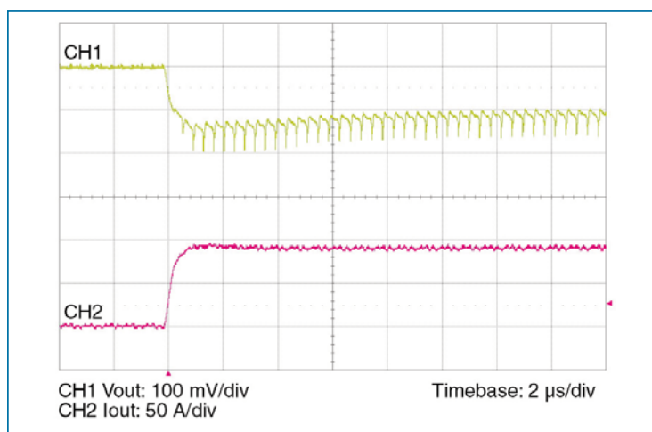
Figure 10 — 0-90 A load step with 100 \mu F input capacitor and no output capacitor.
