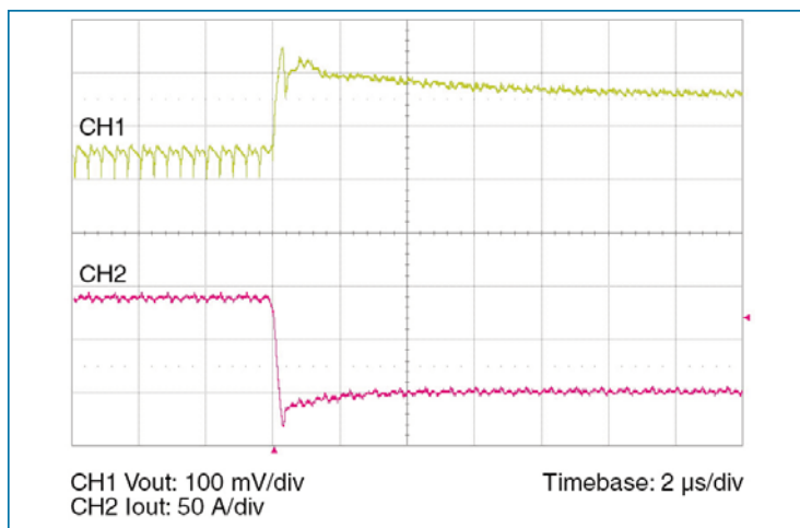
Figure 11 — 90-0 A load step with 100 \mu F input capacitor and no output capacitor.
