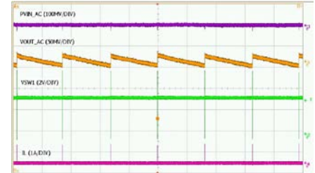
Voltage Ripple (V IN =5.5V, I O =0A)
