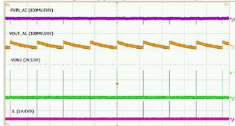
Voltage Ripple (V IN =3V, I O =0A)
