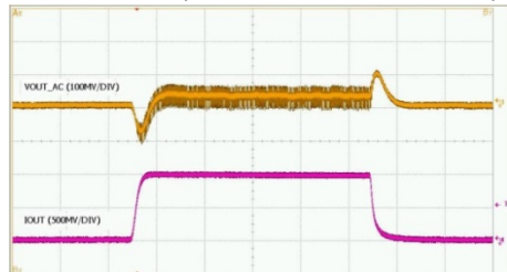
Load Transient (V IN =3.8V, PWM, I O =0A to 1A)
