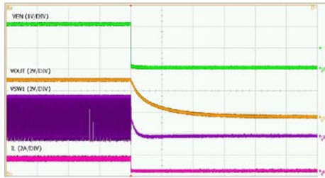
Shutdown through Enable 1A Load, V IN =3.8V
