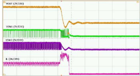
Short Circuit V IN =3.8V, 2A Load
