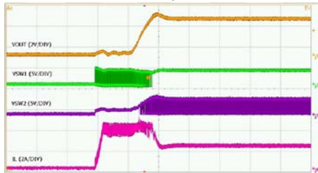
Short Circuit Recovery V IN =3.8V, 2A Load
