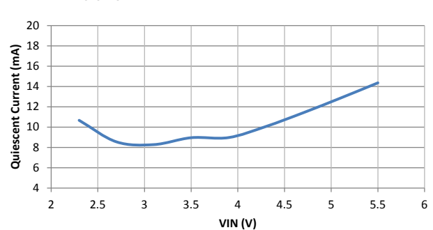
Supply Current (Quiescent), PWM
