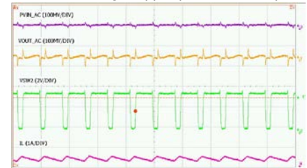
Voltage Ripple (V IN =3V, I O =2A)
