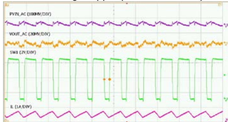
Voltage Ripple (V IN =5.5V, I O =2A)
