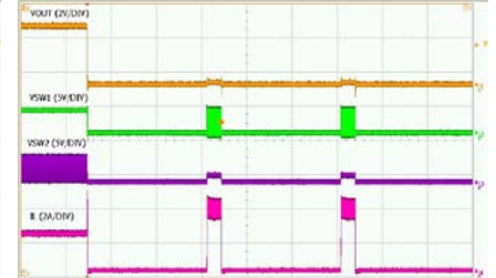
Short Circuit V IN =3.8V, 2A Load
