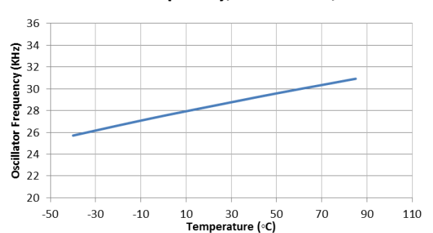
Oscillator Frequency, Vout=3.4V, USM
