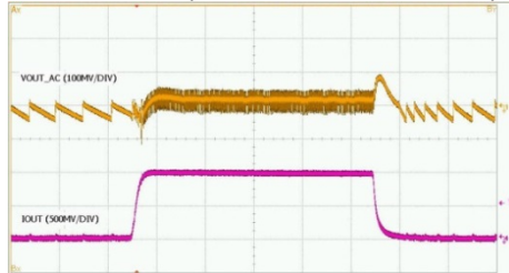
Load Transient (V IN =3.8V, PFM, I O =0A to 1A)
