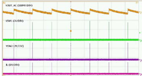
Voltage Ripple (V IN =3.8V, I O =0A)
