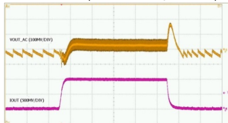
Load Transient (V IN =3V, PFM, I O =0A to 1A)
