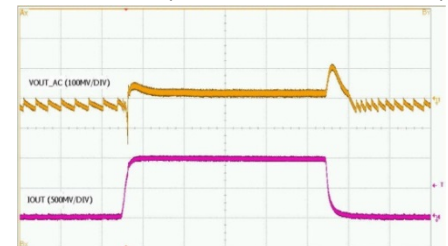
Load Transient (V IN =5.5V, PFM, I O =0A to 1A)
