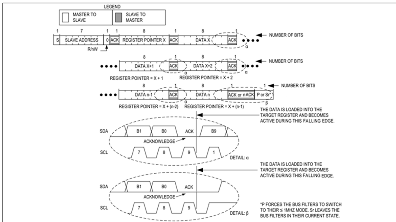
Figure 8 Writing to Sequential Registers X to N
