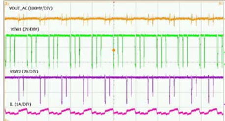
Voltage Ripple (V IN =3.8V, I O =2A)
