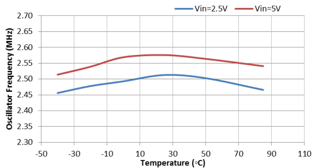
Oscillator Frequency, Vout=3.4V
