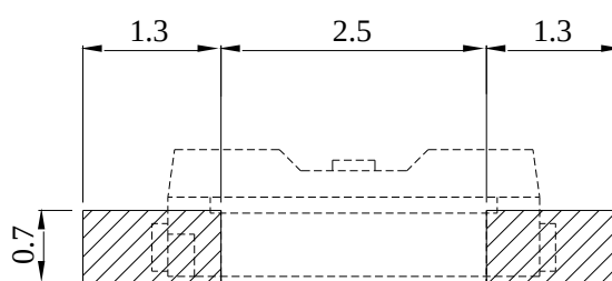
Recommended soldering pad design
