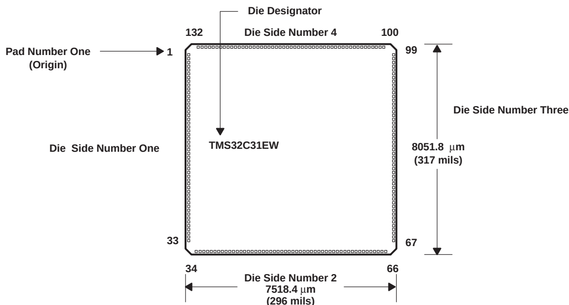
Figure 2. '320C31KGD Die Numbering Format (See Table 1)
